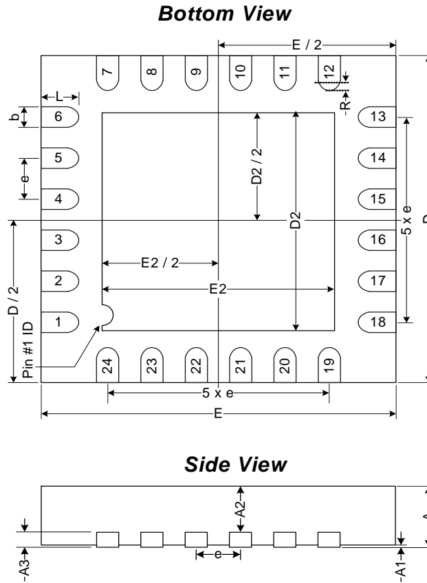
Figure 14. 24-Pin QFN Mechanical Diagram
